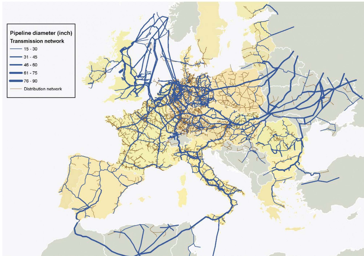
FIG. 1. (Color online) European gas pipeline network. We show the transmission network [blue (dark gray) pipelines] overlaid with the distribution network [brown (light gray) pipelines]. Link thickness is proportional to the pipeline diameter. We projected the data with the Lambert azimuthal equal area projection [17]. Background colors identify EU member states.
