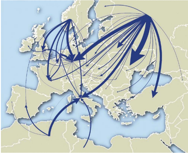
FIG. 2. (Color online) Network of international gas trade movements by pipeline [19]. Link thickness is proportional to the annual volume of gas traded.
