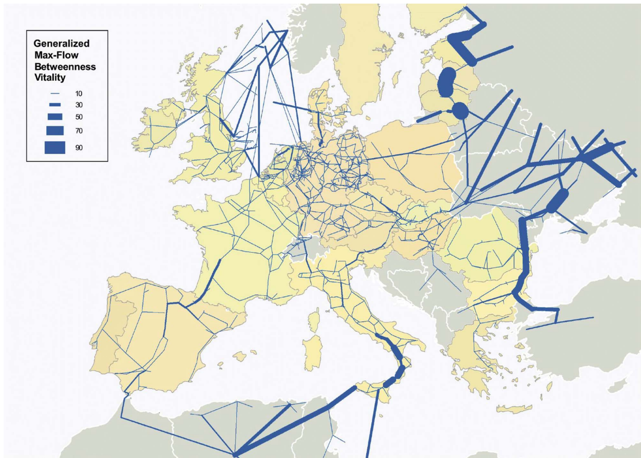
FIG. 8. (Color online) Trans-European natural gas network. Link thickness is proportional to the generalized max-flow betweenness vitality [see Eq. (4), where the sets K and L are countries and the values of T_{K,L} are taken from the data in Fig. 2]. Pipelines close to the major sources tend to have high values of generalized vitality because this is where the network bottleneck is located. Pipelines along sparse interconnections between larger parts of the network (e.g., the Spanish-French border) also tend to have high values of generalized vitality, when compared to neighboring pipelines.
