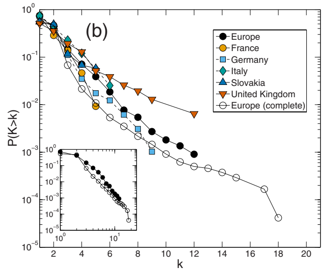
FIG. 3. (Color online) (a) Plot of the number L of links versus the number N of nodes for the transmission and complete (i.e., transmission and distribution) natural gas networks of the countries analyzed. The three largest national transmission and complete networks are also labeled (Germany, UK, and Italy). (b) Plot of the complementary cumulative degree distribution of the European gas networks, together with national transmission gas networks larger than 100 pipelines. The inset shows the degree distribution of the European complete and transmission networks on a double-logarithmic scale, highlighting the presence of fat tails on the degree distribution of the complete gas pipeline network.
