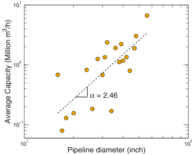
FIG. 4. (Color online) Plot of the digitized GTE pipeline capacity versus the pipeline diameter on a double-logarithmic scale. We digitized the European gas network map from GTE and assigned the GTE capacities to pipelines in the Platts data set. The straight line is a regression to the data, which corresponds to c=ad^\alpha with \alpha=2.46 .
